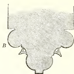
Fig. 35. Diagonal Rib, great vault.
